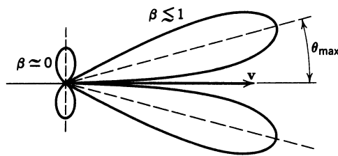
Figure 14.4 Radiation pattern for charge accelerated in its direction of motion. The two patterns are not to scale, the relativistic one (appropriate for \gamma \sim 2 ) having been reduced by a factor \sim 10^2 for the same acceleration.
