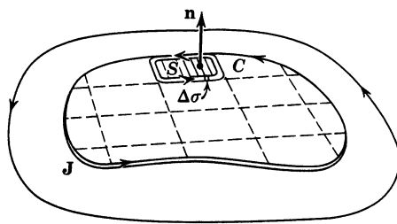
Figure 5.20 Distribution of current density broken up into elemental current loops.
