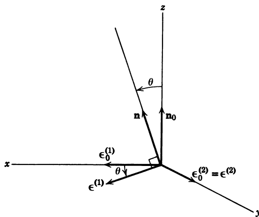
Figure 10.1 Polarization and propagation vectors for the incident and scattered radiation.
