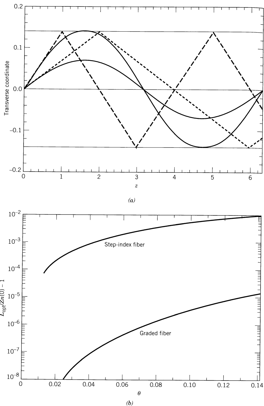
Figure 8.12 (a) Rays at critical angles \theta_{\text{max}} and \theta_{\text{max}}/2 in a simple fiber with \Delta = 0.01 (dashed curves) and a graded fiber of the same radius a , critical angle, and central index, but with a Gaussian profile, n(x) = n_1 e^{-x^2/b^2} for 0 < x < a , ( b \approx a/\sqrt{\Delta} ) and n(x) = n_0 for x > a . Note the difference in scales. Units are such that a = \theta_{\text{max}} \approx \sqrt{2}/10 . (b) Differences in optical path length (divided by the axial index of refraction) and actual length along a fiber, [L_{\text{opt}}/n(0)Z - 1] , for a simple two-index fiber with \Delta = 0.01 and the Gaussian-graded fiber of (a); \theta_{\text{max}} = \sqrt{2}/10 . The compensation from faster phase velocity at larger excursions away from the axis in the graded fiber is striking.
