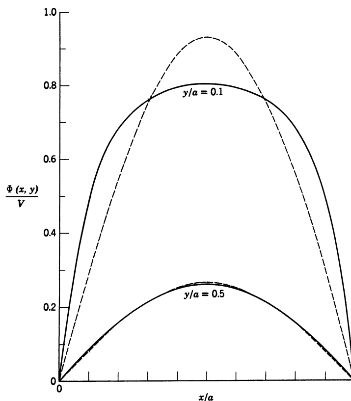
Figure 2.11 Potentials at y/a = 0.1, 0.5 (along the dashed lines of Fig. 2.10) as functions of x/a . The solid curves are the exact solution; the dashed curves are the first term in the series solution (2.61).
