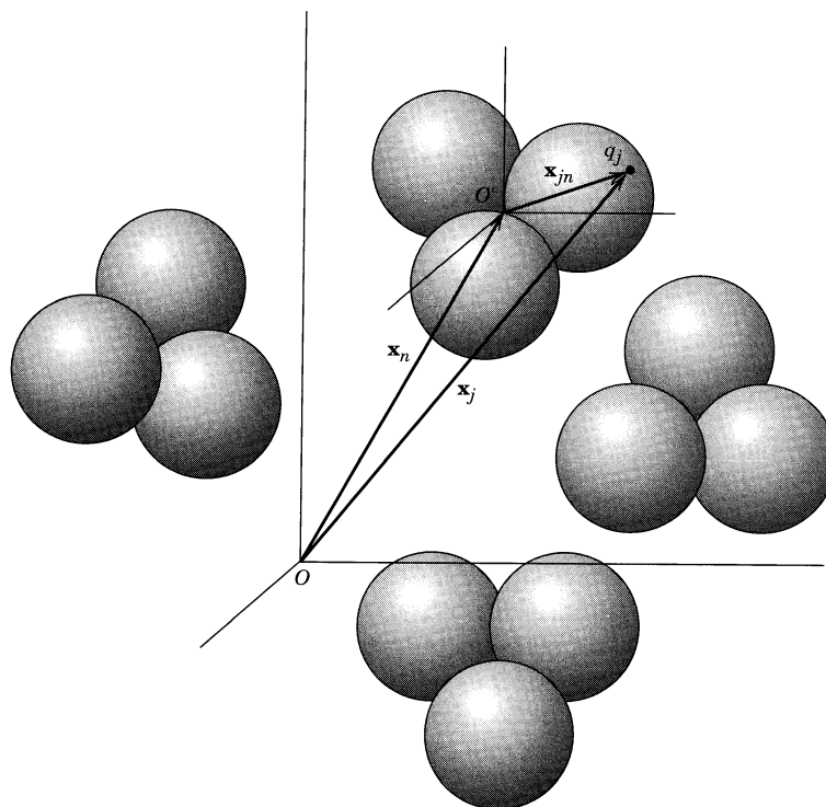
Figure 6.2 Coordinates for the n th molecule. The origin O' is fixed in the molecule (usually it is chosen at the center of mass). The j th charge has coordinate \mathbf{x}_{jn} relative to O' , while the molecule is located relative to the fixed (laboratory) axes by the coordinate \mathbf{x}_n .
