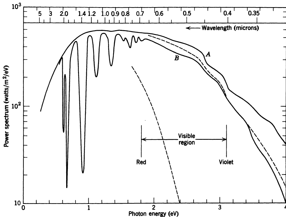
Figure 10.4 Power spectrum of solar radiation (in watts per square meter per electron volt) as a function of photon energy (in electron volts). Curve A is the incident spectrum above the atmosphere. Curve B is a typical sea-level spectrum with the sun at the zenith. The absorption bands below 2 eV are chiefly from water vapor and vary from site to site and day to day. The dashed curves give the expected sea-level spectrum at zenith and at sunrise-sunset if the only attenuation is from Rayleigh scattering by a dry, clean atmosphere.
