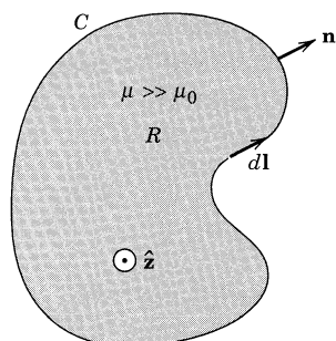
Figure 5.17 Cross section of a long, highly permeable cylindrical conductor with current flow along its length.
