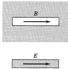
Figure 10.11 Equivalent radiators according to Babinet's principle.
