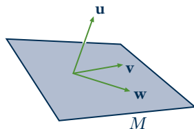
\{\mathbf{u}, \mathbf{v}, \mathbf{w}\} independent
