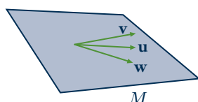
\{\mathbf{u}, \mathbf{v}, \mathbf{w}\} not independent
