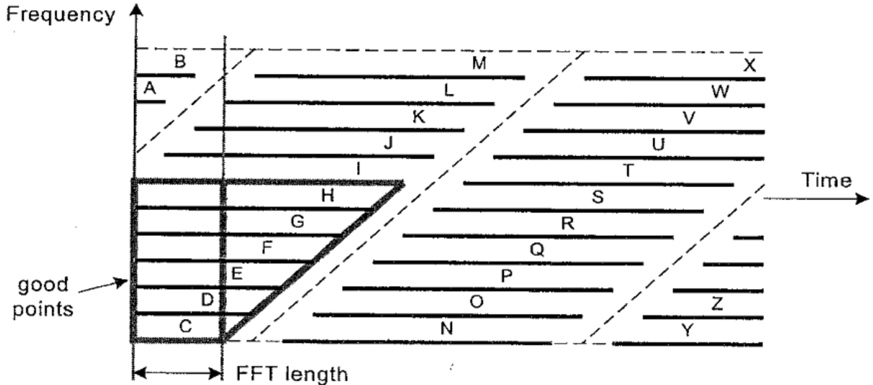
Figure 9.5: Frequency versus time characteristics of multiple targets, illustrating the application of the first FFT.
