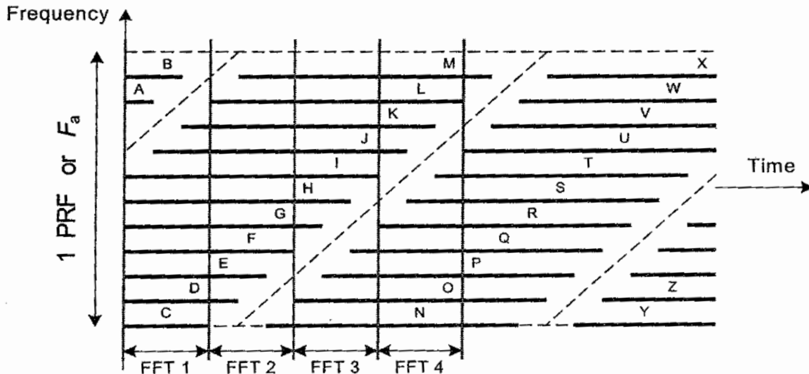
Figure 9.10: Frequency versus time characteristics of multiple targets, illustrating how additional FFTs can be placed between existing FFTs.
