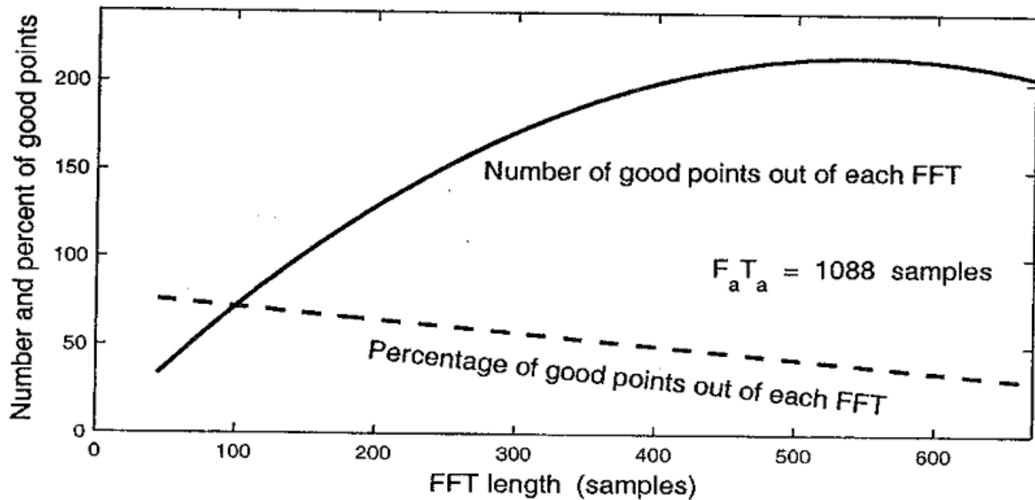
Figure 9.6: The number of good points in the FFT output versus the FFT length.
