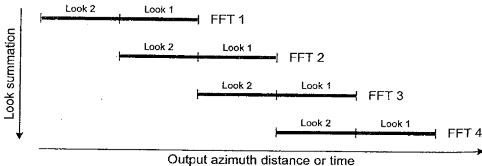
Figure 9.12: Division of the good FFT output points into looks, and alignment of the looks before summation, to form a contiguous multilook image.
